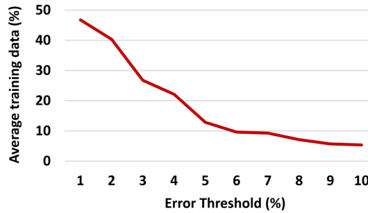
Fig. 14. Average training data required with varying error threshold for all benchmarks. e.g., by using 12.86% training data, we can achieve results within 5% error margin.
