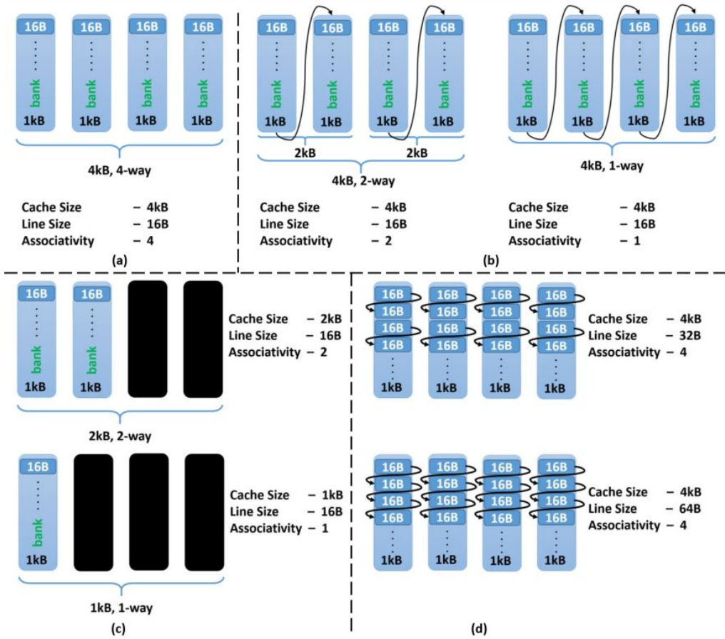
Fig. 2. Cache configurability of a 4kB cache arranged as 4 banks. (a) base cache layout with 4 banks, (b) change of associativity by way concatenation, (c) change of cache size by shutting down ways, (d) change of line size by fetching subsequent blocks and storing them in subsequent cache blocks.
