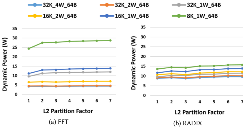
Fig. 6. NoC dynamic power consumption with different DL1 configurations and L2 partition factors. L1 cache is fixed at 32K_2W_64B.
