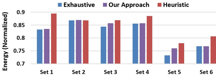
Fig. 16. Energy consumption observed compared to the Base cache configuration across all profile table generation techniques. Goal is to get results similar to exhaustive approach.
