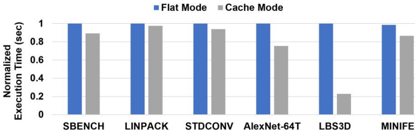
Fig. 8. Execution time variation in Cache vs Flat memory modes in Intel Xeon Phi 7210 processor.
