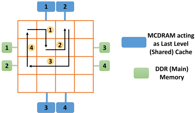
Fig. 10. Traffic model in Cache memory mode in KNL architecture in case of an L1 and MCDRAM miss: (1) L1 cache miss. Memory request injected on the network to check the tag directory, (2) request forwarded to MCDRAM which acts as a cache after miss in tag directory, (3) request forwarded to memory after miss in MCDRAM, (4) data read from memory and sent to the requester.
