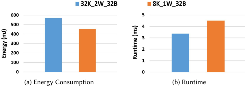
Fig. 5. Energy consumption and runtime of two cache configurations running FFT. The choice of a specific configuration presents a trade-off between energy savings and performance overhead.
